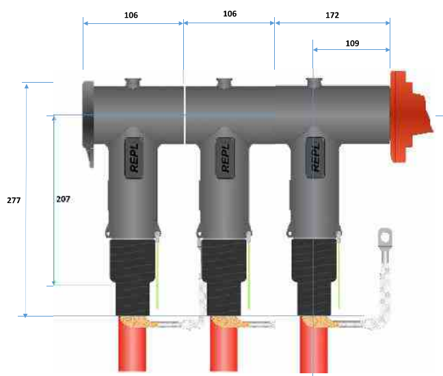
2 X RPCBT-24C installed in back of RPCT-24C
